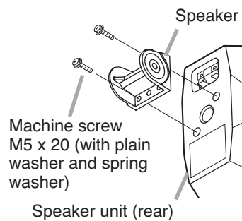
[Vertical speaker installation]
