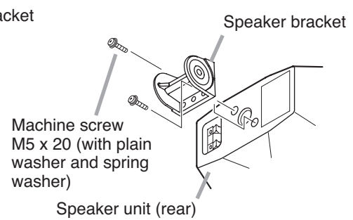
[Horizontal speaker installation]
